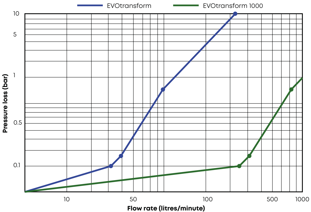
EVOtransform performance diagram
